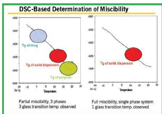
Fig. 5: Thermodynamic and Kinetic Stabilization of Solid Dispersions
