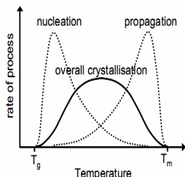
Fig. 4: Overall crystallization rate as a function of temperature. T_g is the glass transition temperature and T_m is the melting temperature
