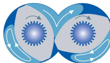
Working principle of co-rotating twin screw extruder
